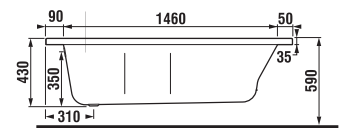
Bathtub for installation with panel
