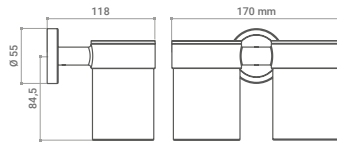
Tooth brush holder duo matte black
