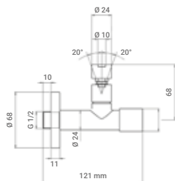
Corner valve with escutcheon matte black
