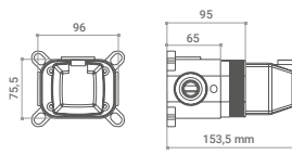
Installation Kit for Concealed Shower 1 Way
