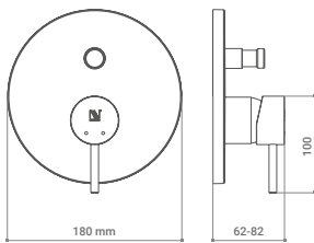
Esthetical assembling kit for Concealed Shower 2 Ways matte black
