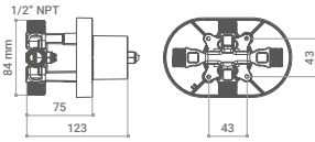
Installation Kit for Concealed Pressure Balance Valve
