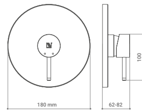
Esthetical assembling kit for Concealed Shower 1 Way matte black
